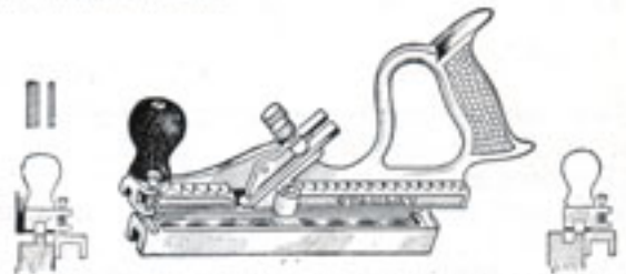
A. Cuts ½ in. groove on boards 1-1½ in. centres on ½ in. .. price 20/- B. .. .. 20/-
