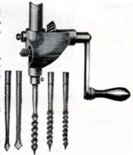
BORING APPARATUS
